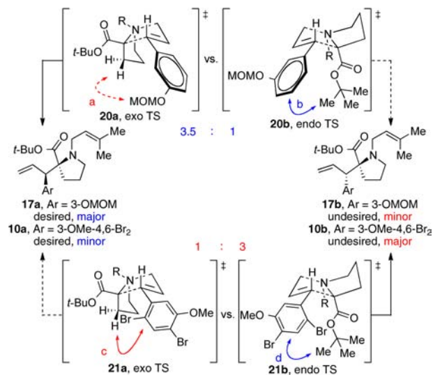
Scheme 4. Rationale for Switch in Diastereoselectivity
