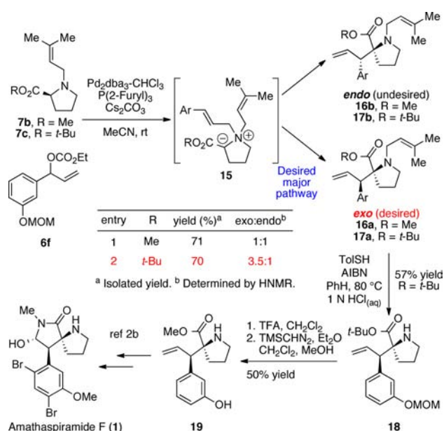
Scheme 3. Switch in Diastereoselectivity for Palladium-Catalyzed Allylic Amination/[2,3]-Rearrangement
